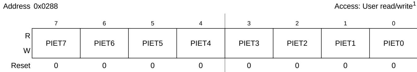
Figure 2-63. Port T Interrupt Enable Register (PIET)
