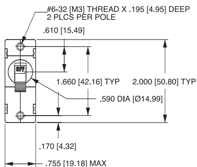
1-POLE (AA1)
