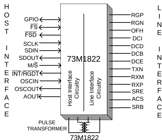
Figure 1: MicroDAA System Block Diagram
