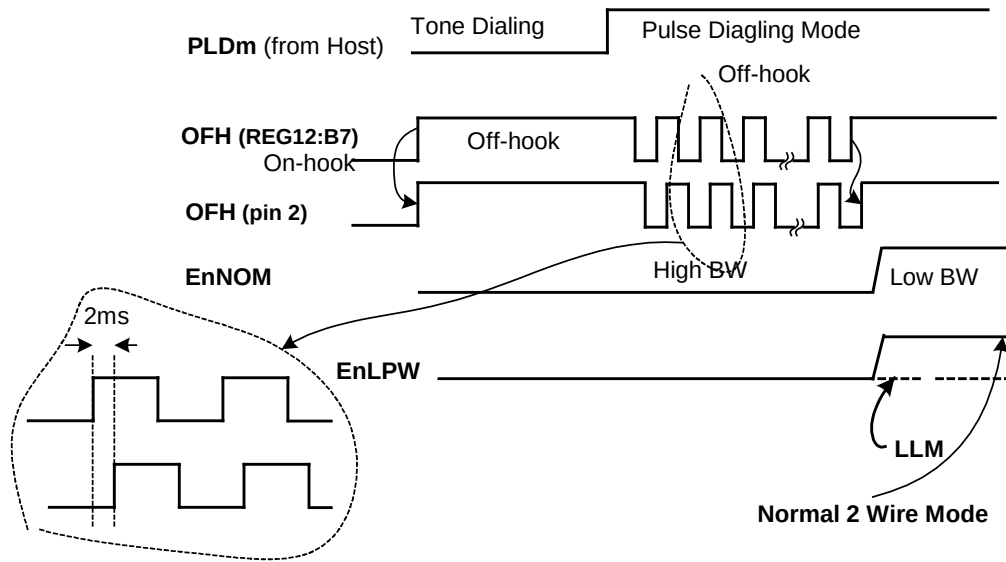
Figure 4: Pulse Dialing Sequence
