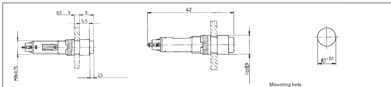
Mounting hole
