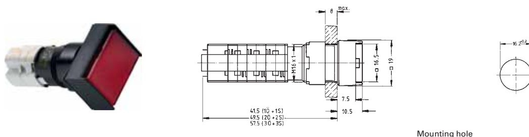
Mounting hole
