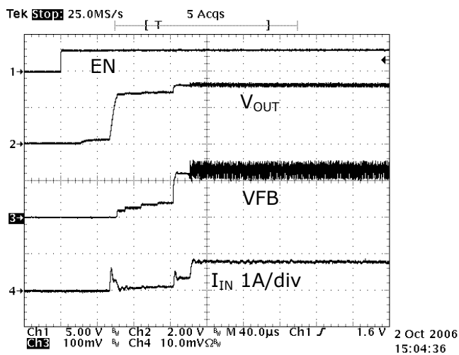
SP7686A Flash Mode 2X, VIN=3.4V
