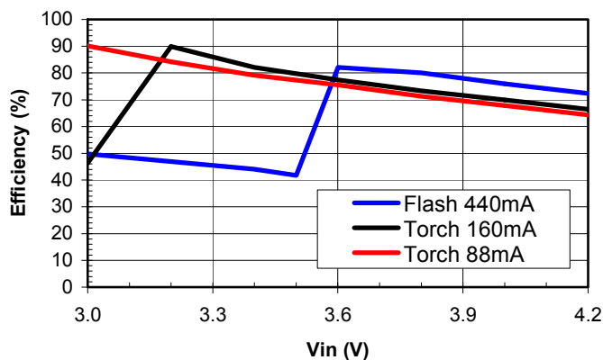
Fig. 6: SP7686 Efficiency
