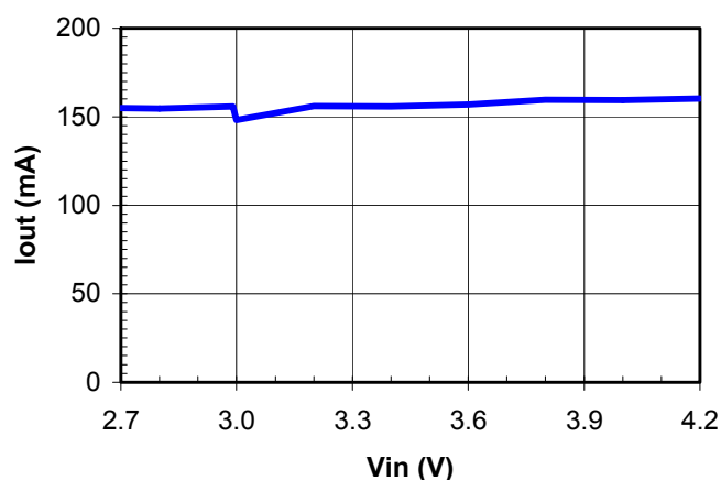
Fig. 14: SP7686A Torch Mode Output Current
