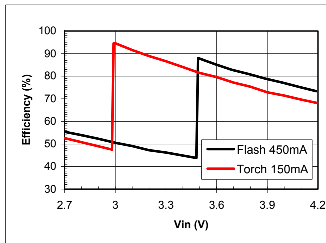
Fig. 12: SP7686A Efficiency
