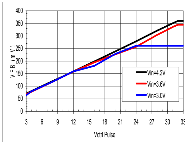
Fig. 3: SP7686 VFB vs CTRL Pulses
