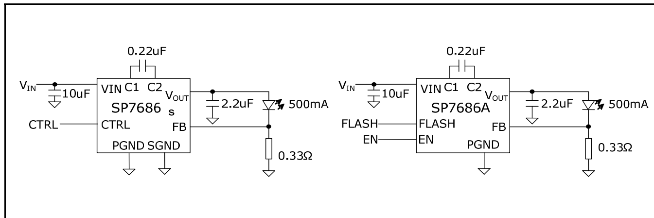
Fig. 1: SP7686 and SP7686A Application Diagrams
