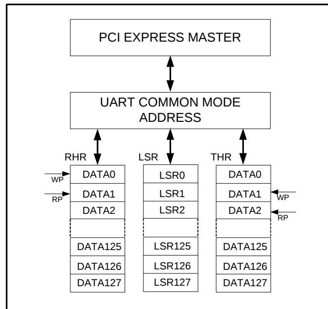
Figure 5-1 Transmit and Receive FIFOs
