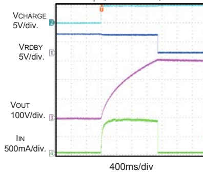
Charging Waveform
