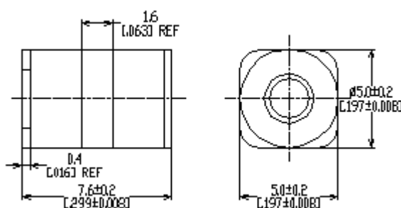
Surface-mount (GTCS35-XXXM-R05)
