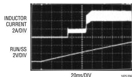
Soft Start: Load Current vs Time
