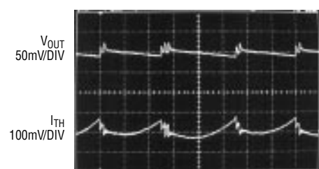
Burst Mode Operation
