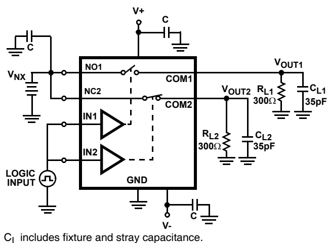
FIGURE 3B. TEST CIRCUIT
