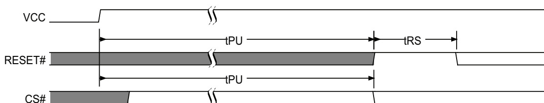
Figure 20. POR followed by Hardware Reset
