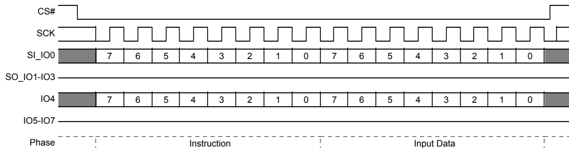
Figure 50. Write VDLR (WVDLR 4Ah) Command Sequence
