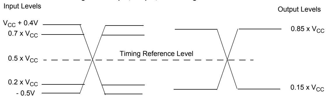
Figure 16. Input, Output, and Timing Reference Levels
