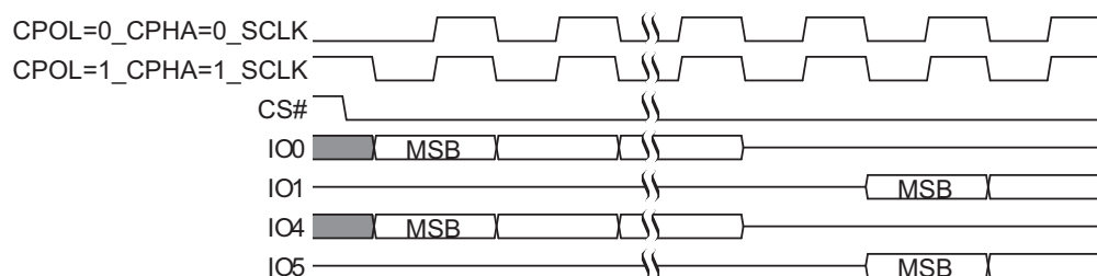
Figure 2. Dual-Quad SPI SDR Modes Supported
