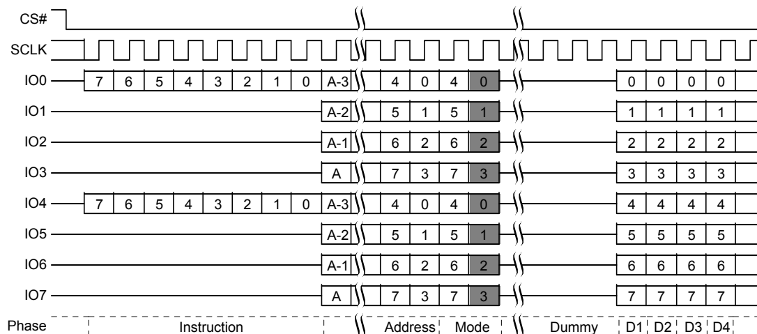
Figure 55. Dual-Quad I/O Read Command Sequence (3-Byte Address, EBh [ExtAdd=0], LC=00b)
