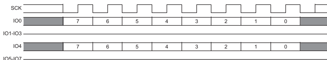
Figure 67. Dual-Quad Erase Resume Command Sequence
