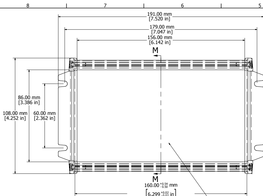
ASSEMBLY - VIEW FROM TOP
