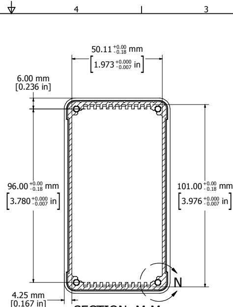
SECTION M-M
