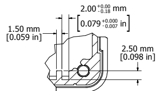
DETAIL N
