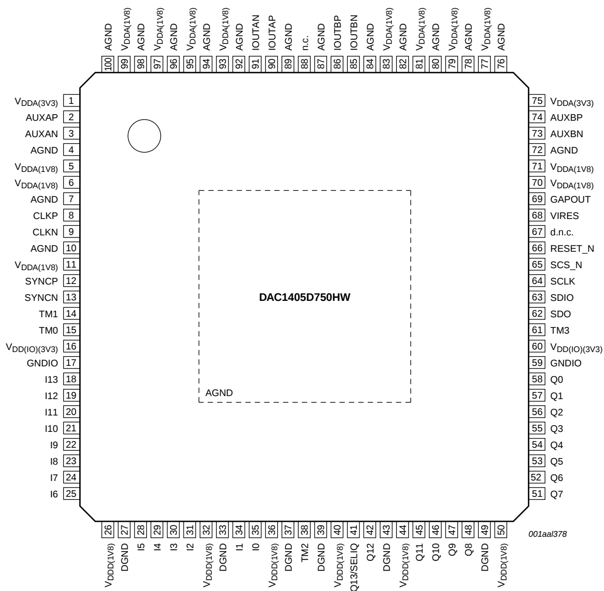
Fig 2. Pin configuration
