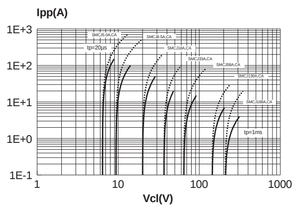
Fig. 4: Clamping voltage versus peak pulse current ( T_{j \text{ initial}}=25^{\circ}\text{C} ). Exponential waveform t_p=20\mu\text{s} & t_p=1\text{ms} .
