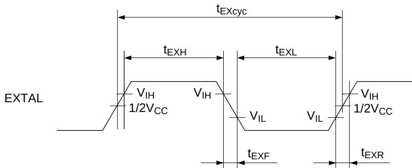
Figure 27.2 Peripheral Clock Timing
