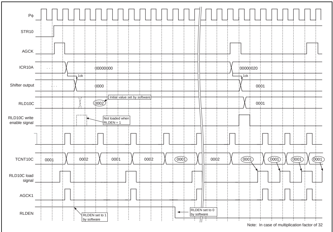
Figure 11.30 TCNT10C Operation
