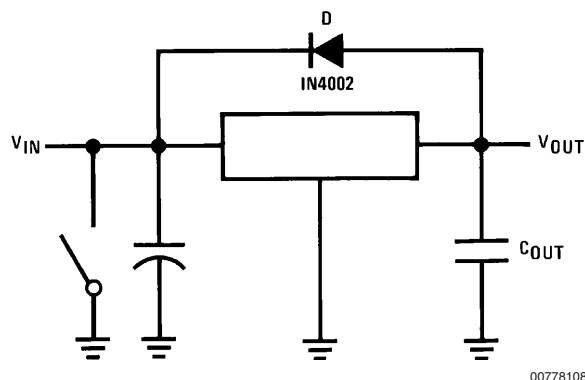
FIGURE 1. Input Short
