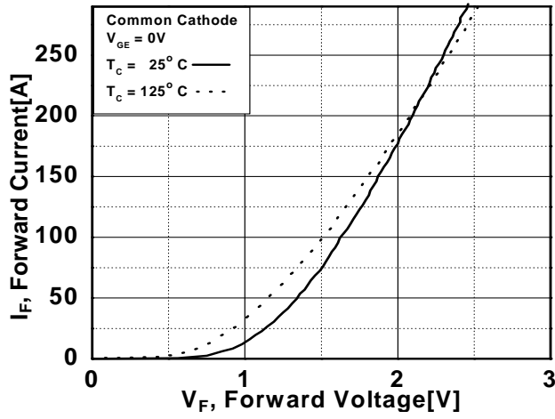
Fig 19. Forward Characteristics
