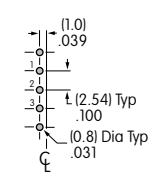
B1 Terminals
