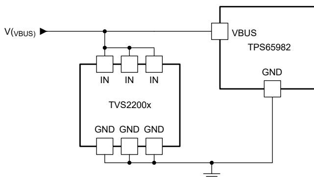
Figure 9-1. TVS2200 Application
