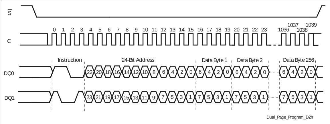
Figure 49. Dual Command Page Program instruction sequence DIO-SPI, D2h
