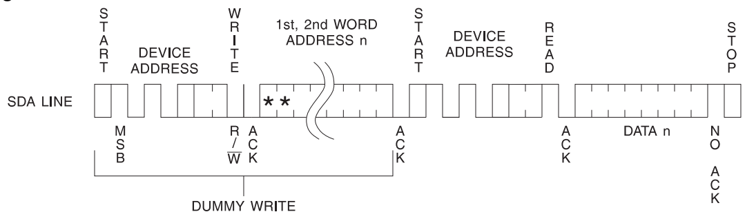
Figure 9-2. Random Read
