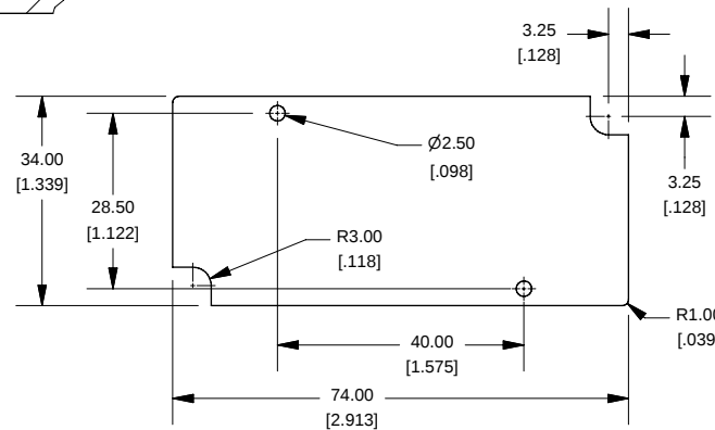
Maximum P.C. Board Size
