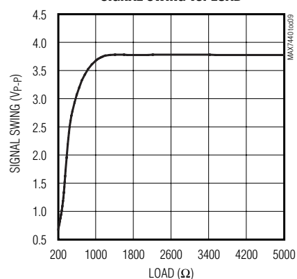
SIGNAL SWING vs. LOAD
