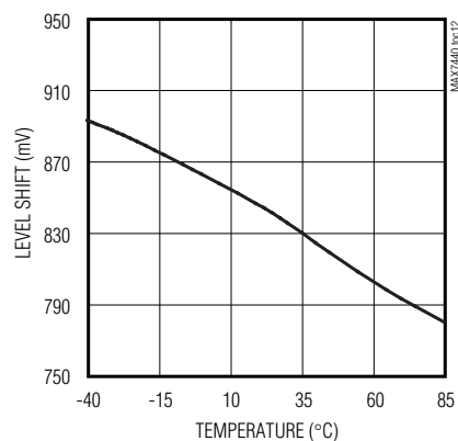
INPUT/OUTPUT LEVEL SHIFT vs. TEMPERATURE
