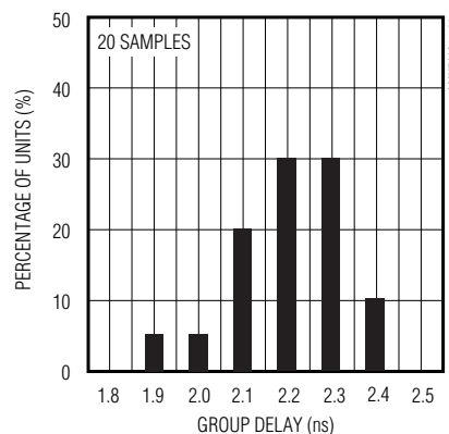
GROUP DELAY MATCHING DISTRIBUTION
