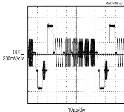
MULTIBURST RESPONSE
