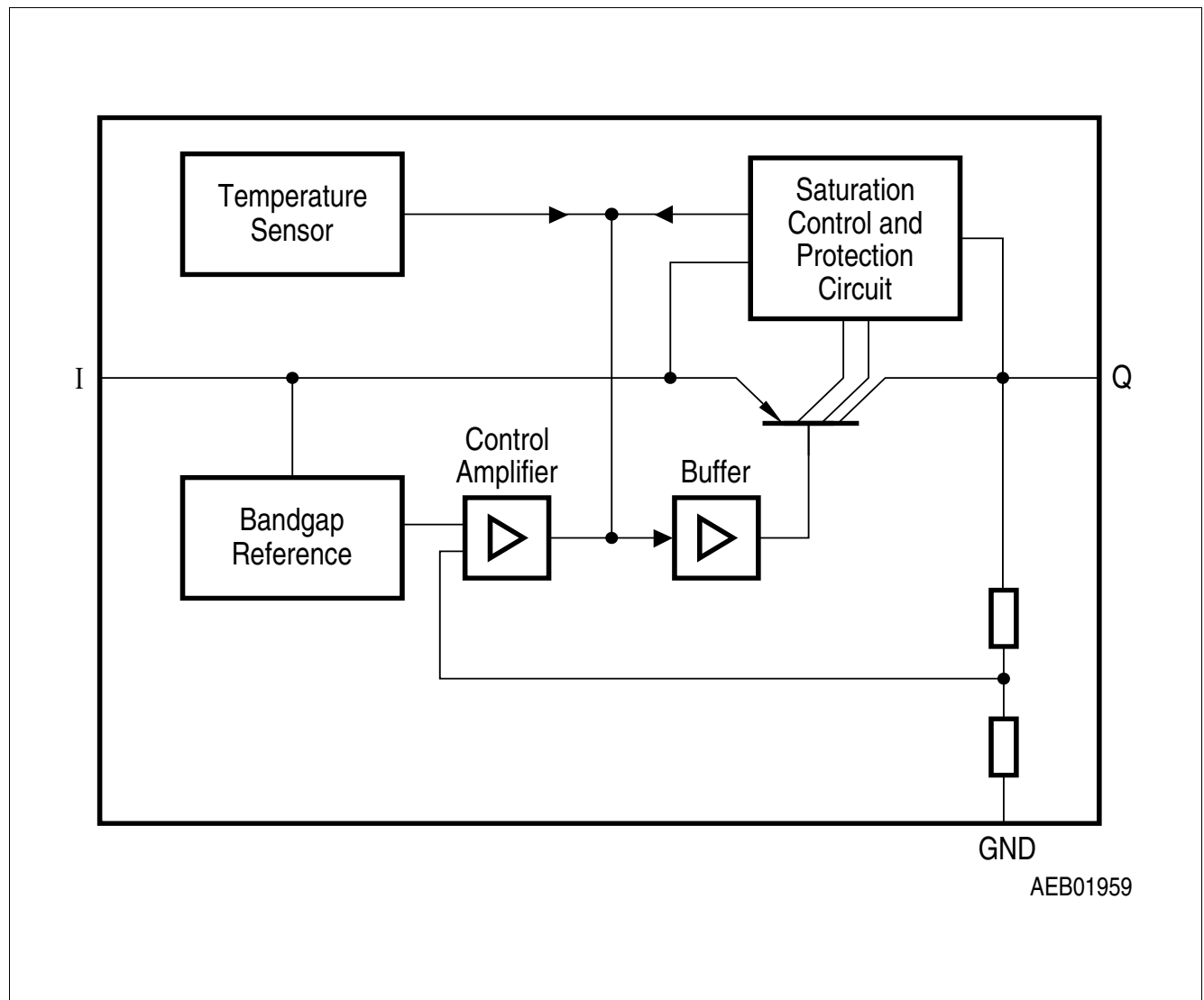
Figure 1 Block Diagram
