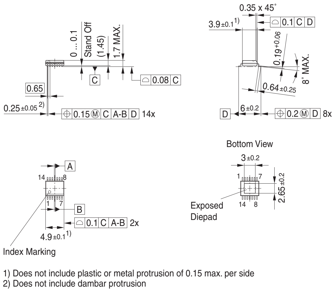
Figure 6 PG-SSOP-14 exposed pad
