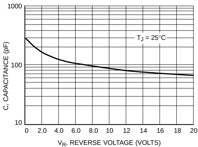
Figure 3. Capacitance
