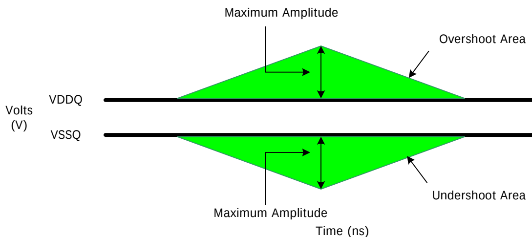
Clock, Data Strobe and Mask Overshoot and Undershoot Definition
