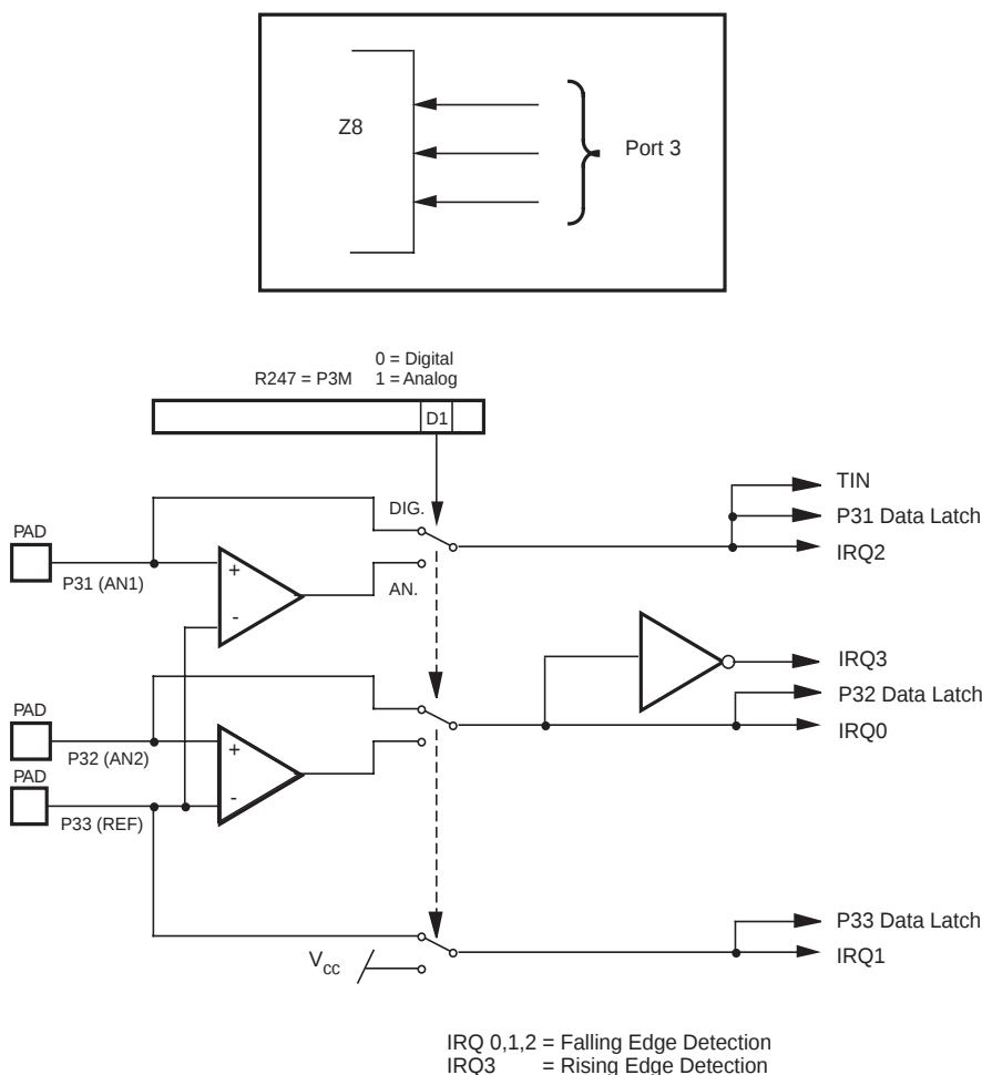
Figure 10. Port 3 Configuration
