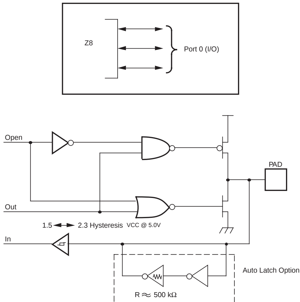
Figure 8. Port 0 Configuration
