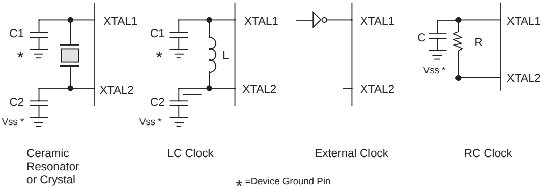
Figure 17. Oscillator Configuration
