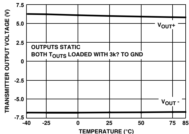
FIGURE 23. RS-232, TRANSMITTER OUTPUT VOLTAGE vs TEMPERATURE
