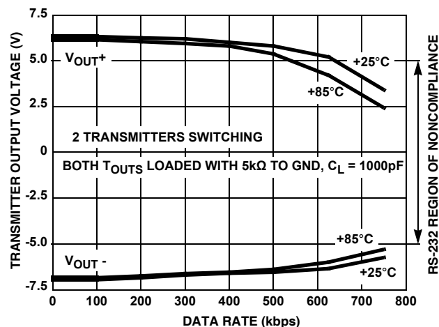
FIGURE 29. RS-232, TRANSMITTER OUTPUT VOLTAGE vs DATA RATE
