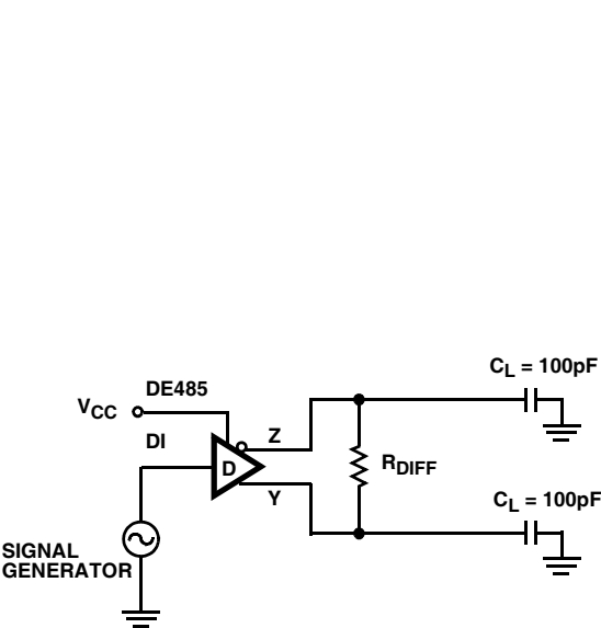
FIGURE 3A. TEST CIRCUIT
