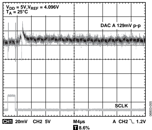
Figure 44. Glitch Upon Exiting Power-Down ( 1\text{ k}\Omega to GND) to Zero Scale, No Load
