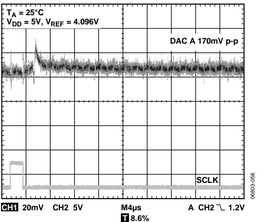
Figure 45. Glitch Upon Exiting Power-Down ( 1\text{ k}\Omega to GND) to Zero Scale, 5\text{ k}\Omega/200\text{ pF} Load
