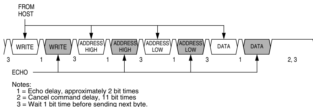
Figure 18-16. Write Transaction
