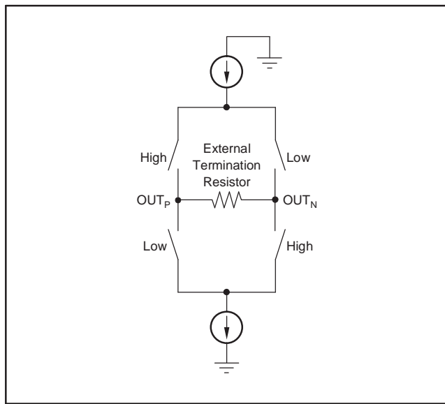
Figure 37. LVDS Buffer
