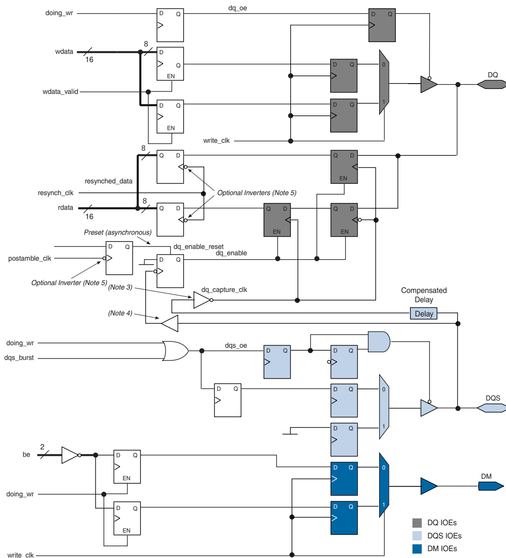
Figure 3-5. Stratix DQS Group Block Diagram (Note 1) (2)
