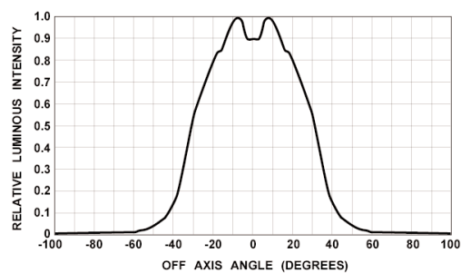
Figure 5d. HPWA(T)-Dx02 Relative Luminous Intensity vs. Off Axis Angle.
