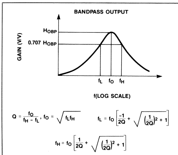
Figure 9. Second-Order Bandpass Characteristics
