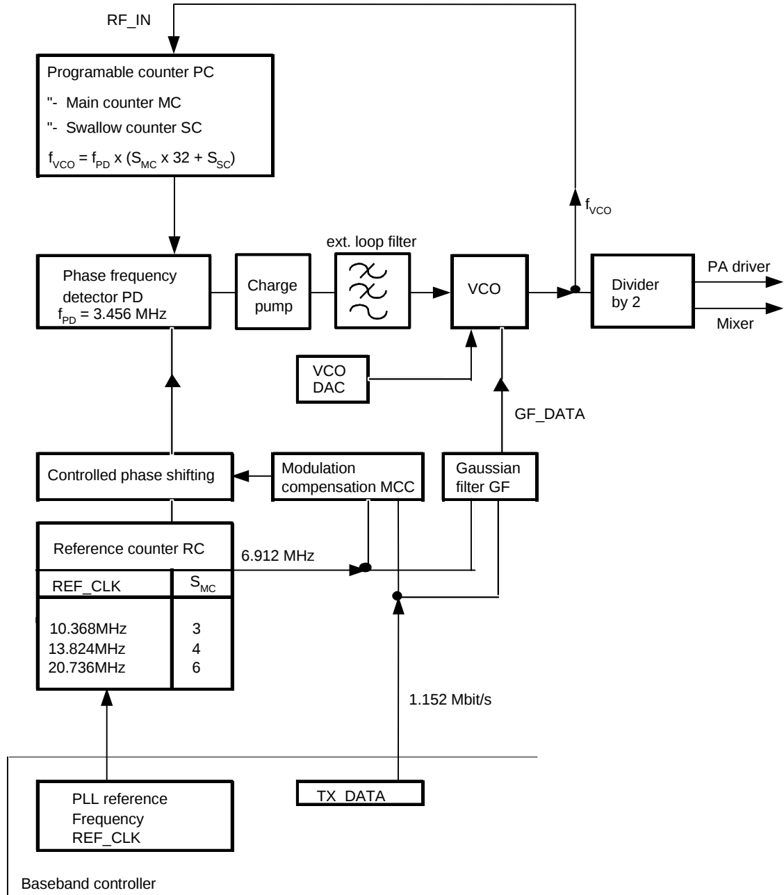
Figure 3. PLL Principle
