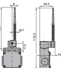
Nylon Actuator with Stainless Steel Spring
