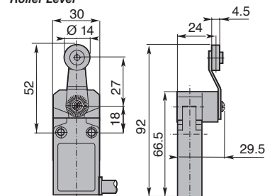
Roller Lever
