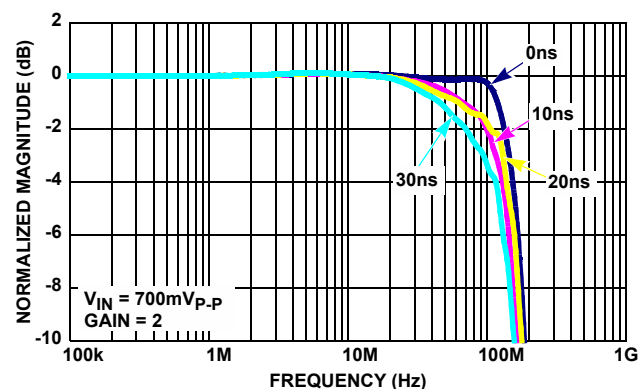
FIGURE 10. ISL59923 FREQUENCY RESPONSE (GAIN = 2)
