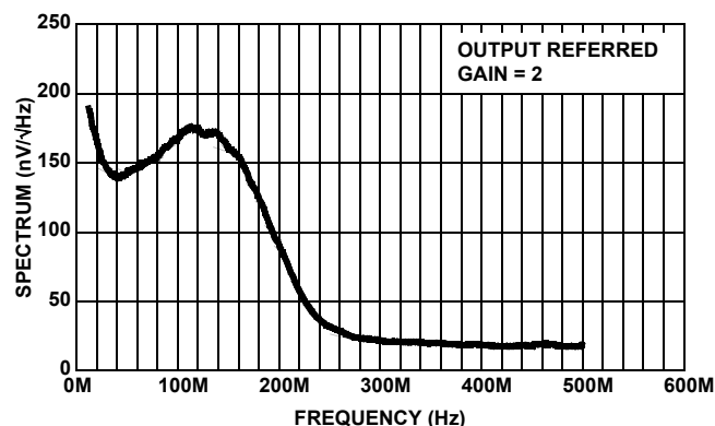
FIGURE 12. ISL59920 NOISE SPECTRUM (10k TO 500MHz)
