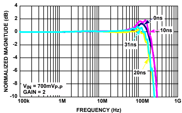
FIGURE 8. ISL59922 FREQUENCY RESPONSE (GAIN = 2)
