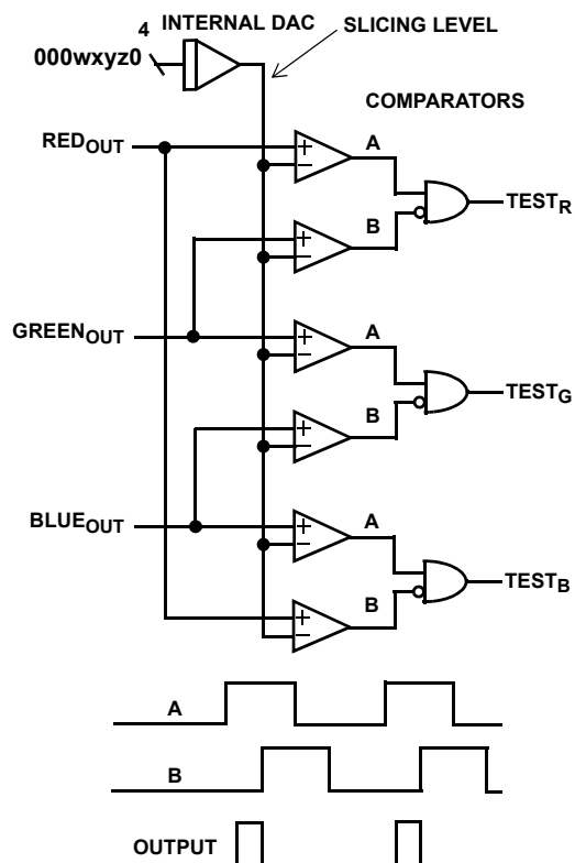
FIGURE 36. DELAY DETECTOR
