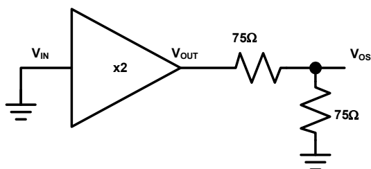
FIGURE 2. V_{OS} MEASUREMENT CONDITIONS
