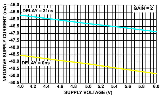
FIGURE 30. ISL59922 I_{SUPPLY-} vs V_{SUPPLY-}
