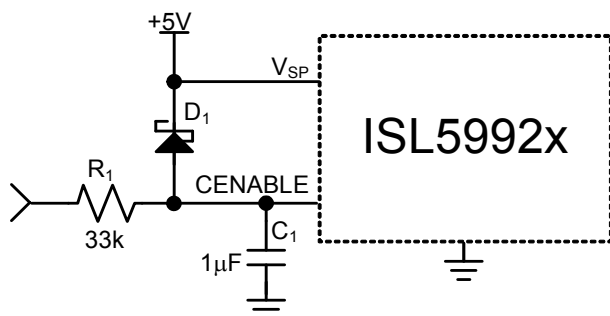
FIGURE 37. CENABLE RC DELAY
