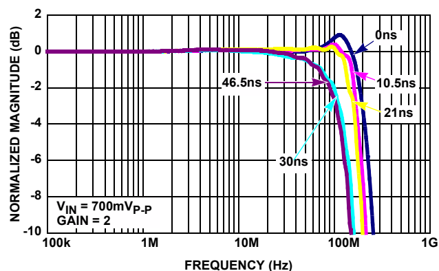
FIGURE 6. ISL59921 FREQUENCY RESPONSE (GAIN = 2)
