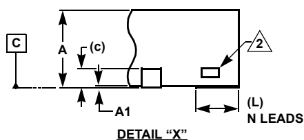
DETAIL "X"
