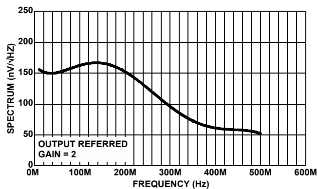
FIGURE 14. ISL59922 NOISE SPECTRUM (10k TO 500MHz)
