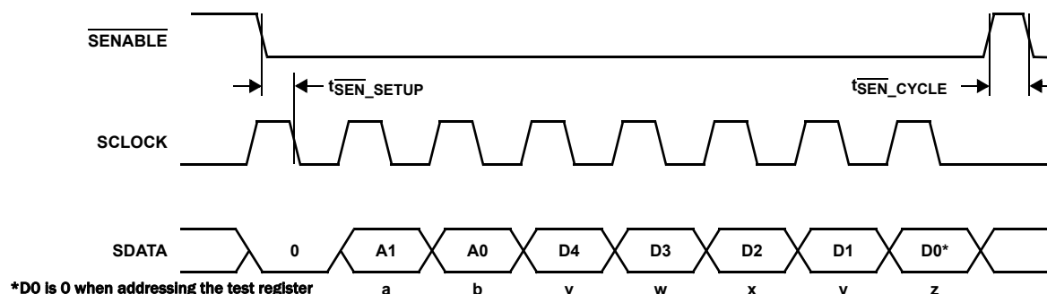
FIGURE 35. SERIAL TIMING
