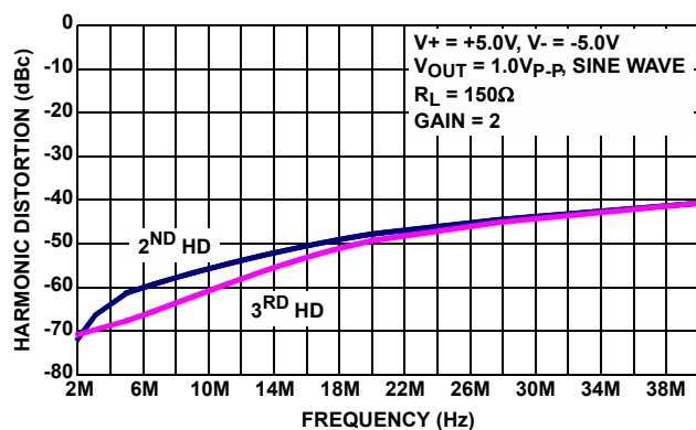
FIGURE 20. HARMONIC DISTORTION vs FREQUENCY
