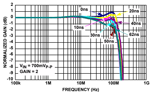
FIGURE 4. ISL59920 FREQUENCY RESPONSE (GAIN = 2)
