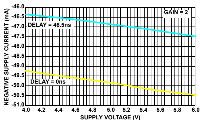
FIGURE 28. ISL59921 I_{SUPPLY-} vs V_{SUPPLY-}
