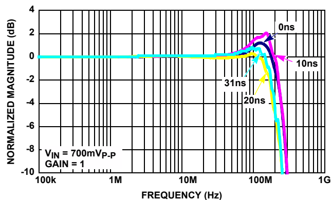
FIGURE 7. ISL59922 FREQUENCY RESPONSE (GAIN = 1)
