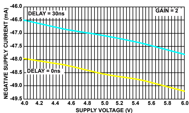
FIGURE 32. ISL59923 I_{SUPPLY-} vs V_{SUPPLY-}
