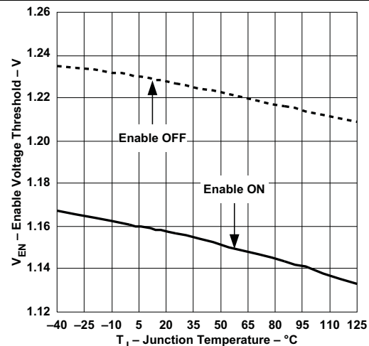
Figure 4. \overline{\text{EN}}x Turnon and Turnoff Threshold vs Temperature
