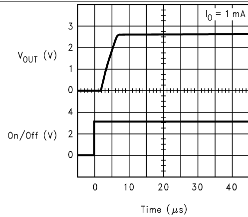
Figure 14. Enable Response
