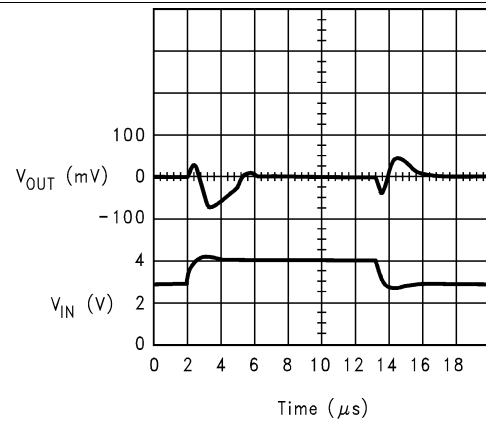
Figure 16. Line Step Response
