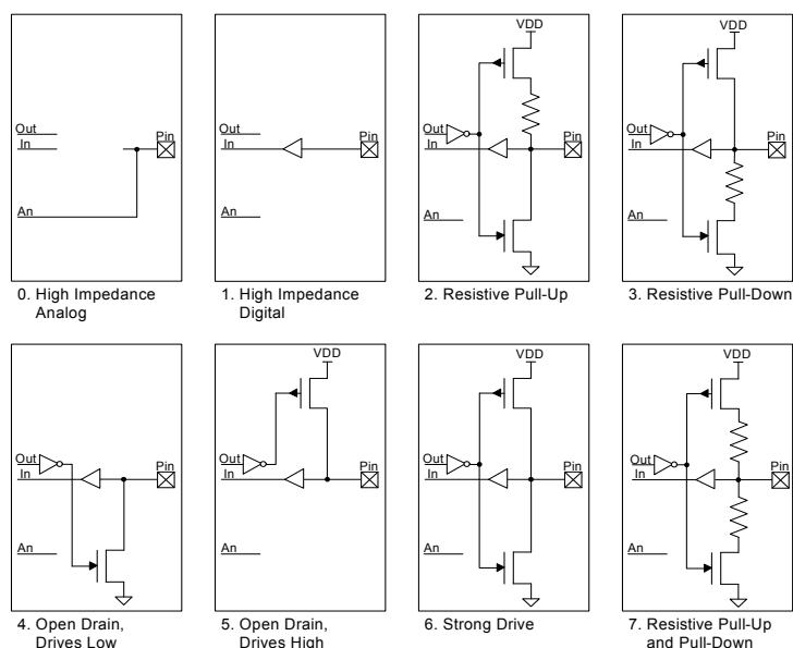
Figure 6-6. Drive Mode
