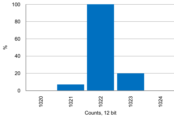
Figure 11-15.SAR ADC Noise Histogram, 1 mps, External Reference
