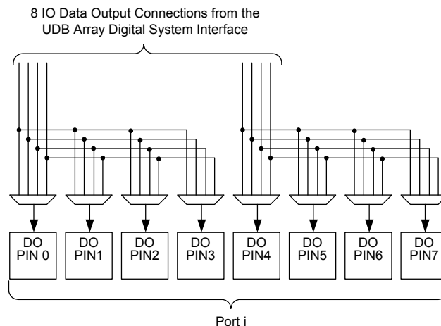
Figure 7-8. I/O Pin Output Connectivity
