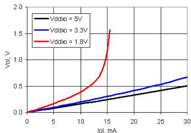
Figure 11-15. GPIO Output Low Voltage and Current
