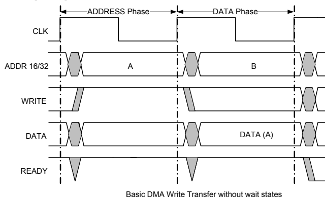
Figure 4-3.DMA Timing Diagram
