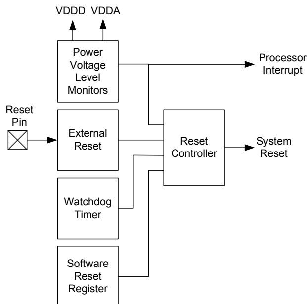
Figure 6-3. Resets
