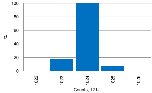
Figure 11-14.SAR ADC Noise Histogram, 1 mps, Internal Reference Bypassed
