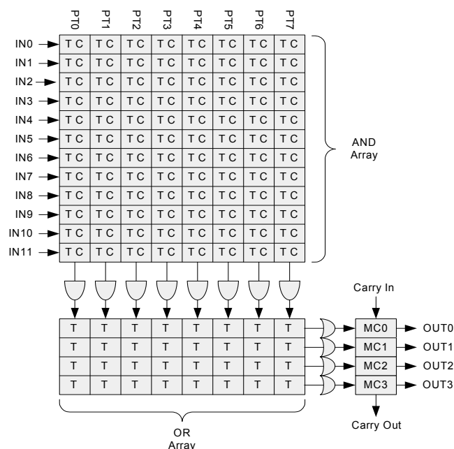
Figure 7-8. PLD 12C4 Structure
