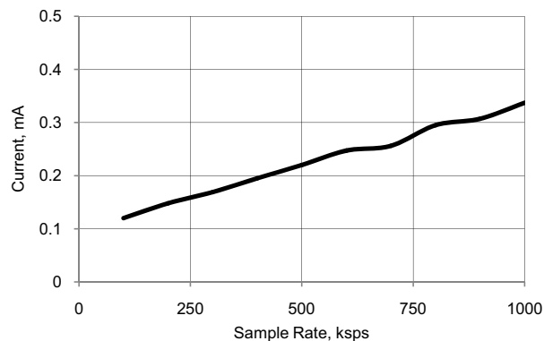
Figure 11-12. SAR ADC I_{DD} vs sps , V_{DDA} = 5\text{ V} , Continuous Sample Mode, External Reference Mode
