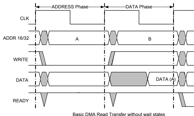
Figure 4-3.DMA Timing Diagram
