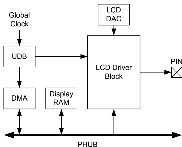
Figure 8-7. LCD System
