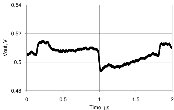
Figure 11-12.VDAC Voltage Noise, 1 V Mode, Fast Mode, V_{DDA} = 5 V
