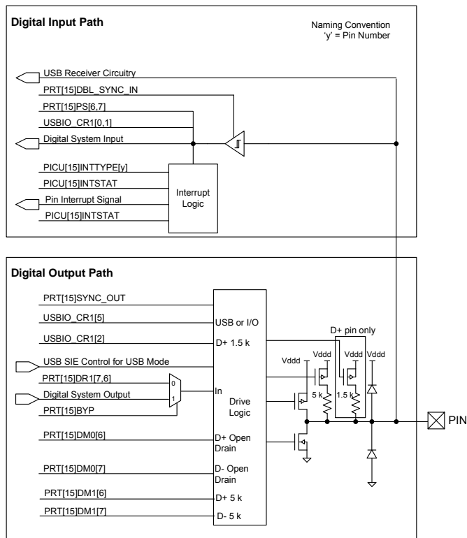
Figure 6-5.USBIO Block Diagram
