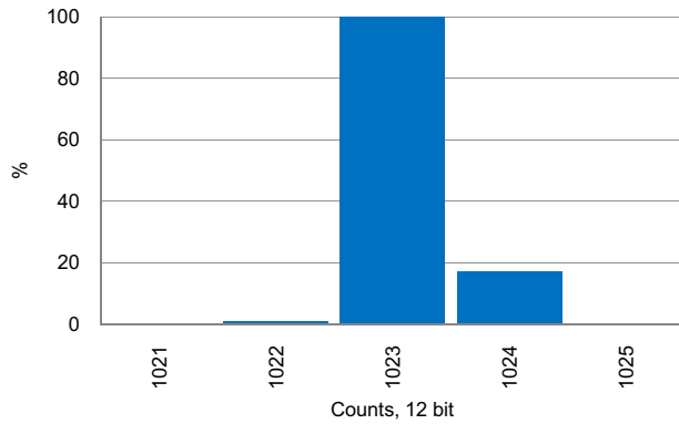
Figure 11-13.SAR ADC Noise Histogram, 100 kps, Internal Reference No Bypass
