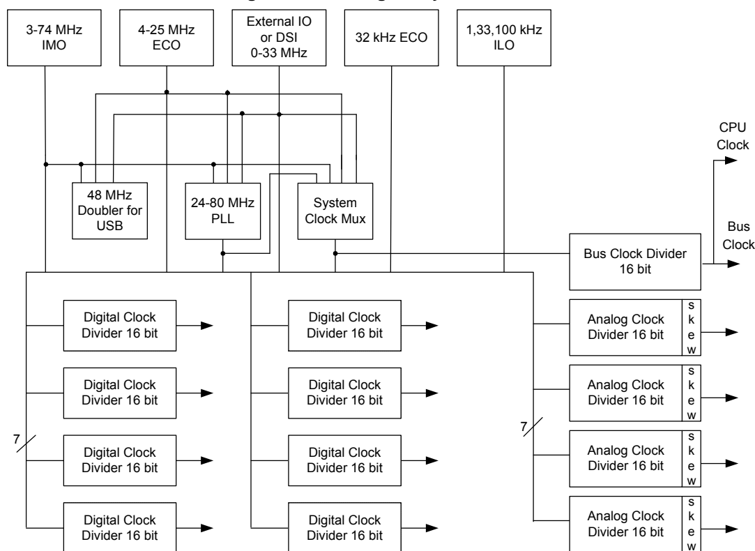
Figure 6-1. Clocking Subsystem
