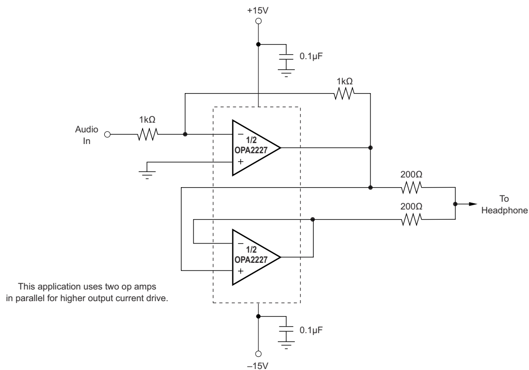
Figure 8-11. Headphone Amplifier
