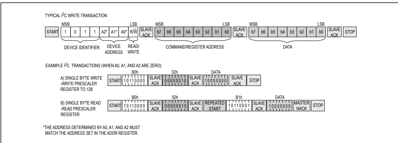
Figure 6. I^2C Transactions
