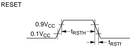
Figure 106 Reset Timing
