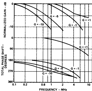
Figure 17. Closed Loop Gain & Phase vs. Frequency
