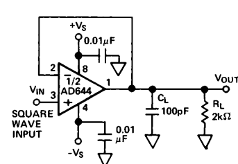
Figure 21c. Unity Gain Follower Pulse Response (Small Signal)
