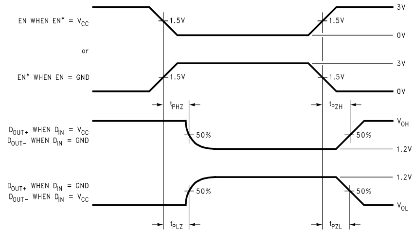
Figure 7. Driver TRI-STATE Delay Waveform
