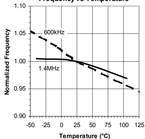
Normalized Channel Frequency vs Temperature
