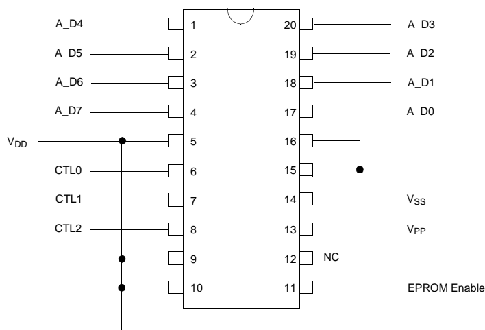
Figure 20-3 Pin Assignment ( HMS1204/2A )
