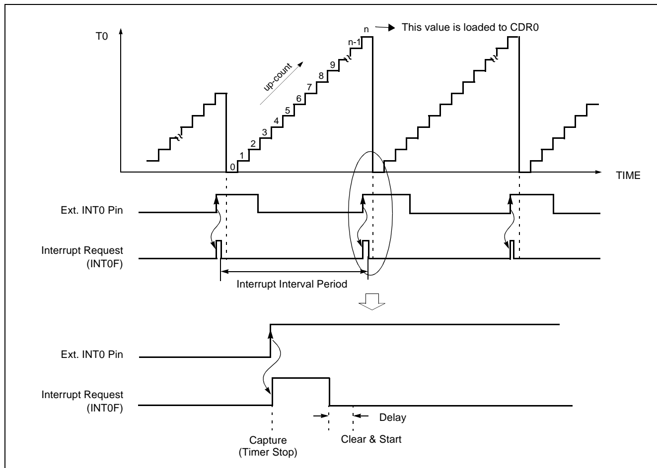
Figure 12-7 Input Capture Operation
