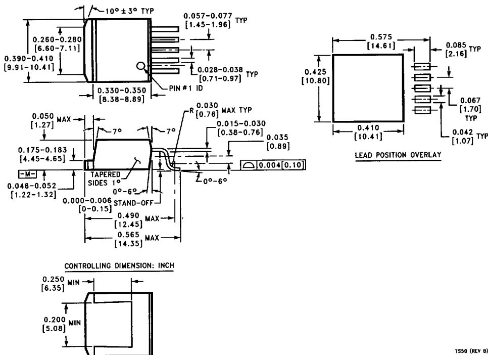
TO-263 5-Lead Plastic Surface Mount Package Order Number LM2941S or LM2941CS NS Package Number TS5B
