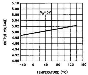
Output Voltage
