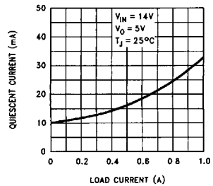
Quiescent Current
