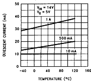
Quiescent Current vs Temperature
