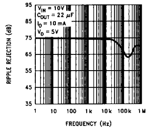
Ripple Rejection
