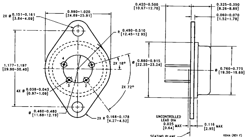
Order Number LM2941K/883 NS Package Number K04A
