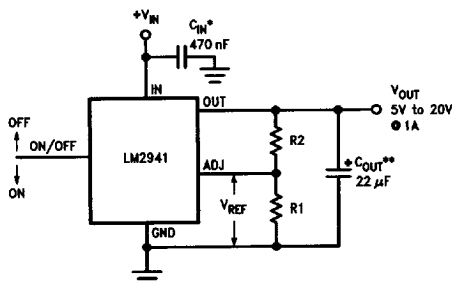
5V to 20V Adjustable Regulator
