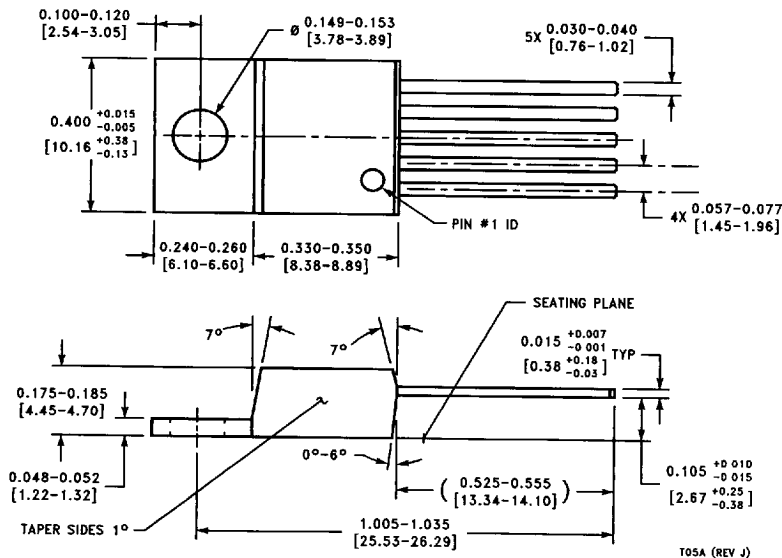
Order Number LM2941T or LM2941CT NS Package Number T05A
