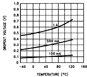
Dropout Voltage vs Temperature
