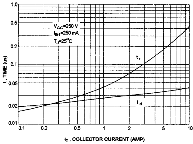
TURN-ON TIME
