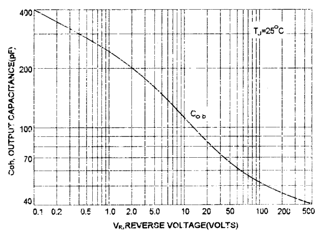
OUTPUT CAPACITANCES
