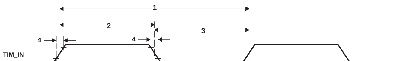
Figure 6-71. Timer Timing
